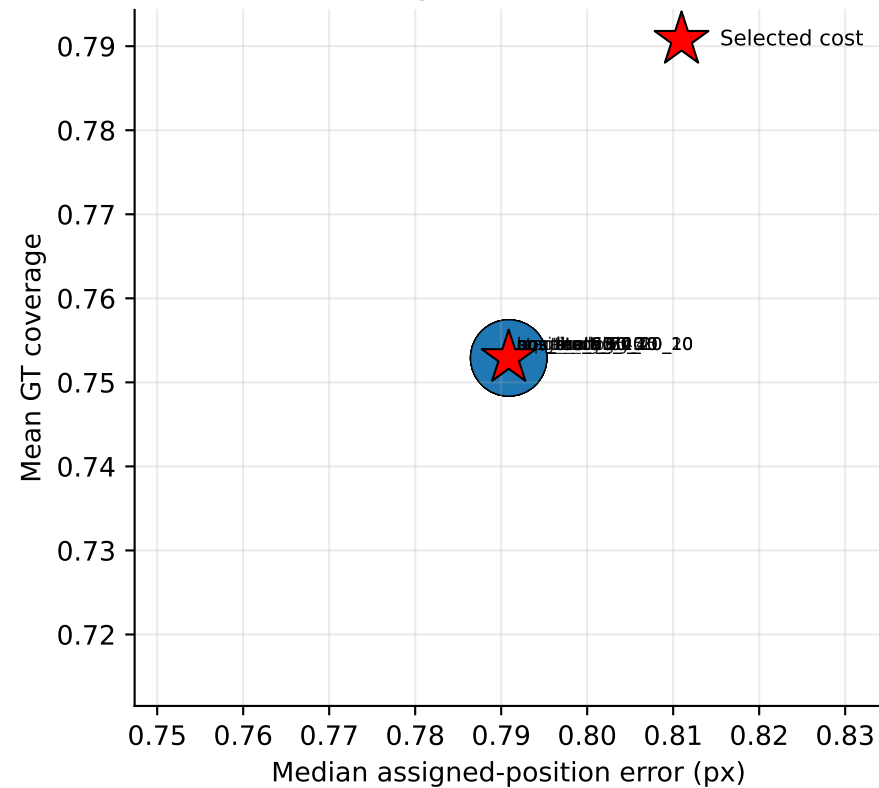
Coverage--error trade-off
