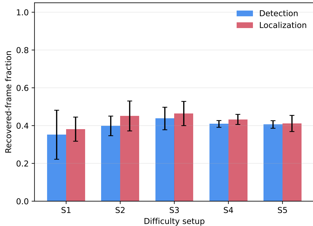
Trajectory coverage
