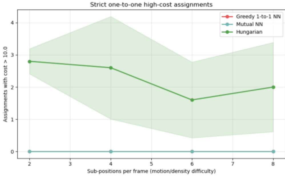
Strict 1-to-1 high-cost
