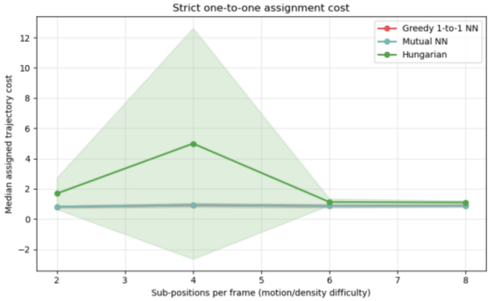
Strict 1-to-1 assignment cost
