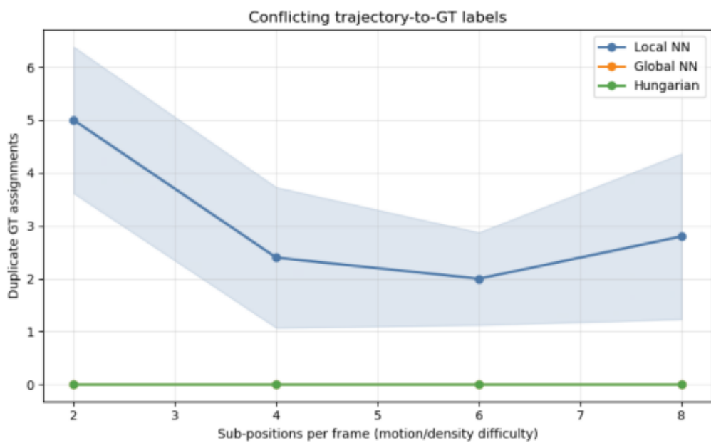
Duplicate GT assignments
