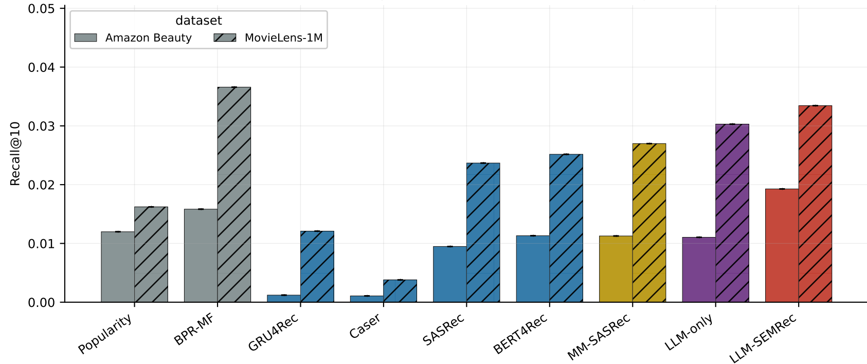
Overall recommendation performance — Recall@10 (full-catalogue ranking)
