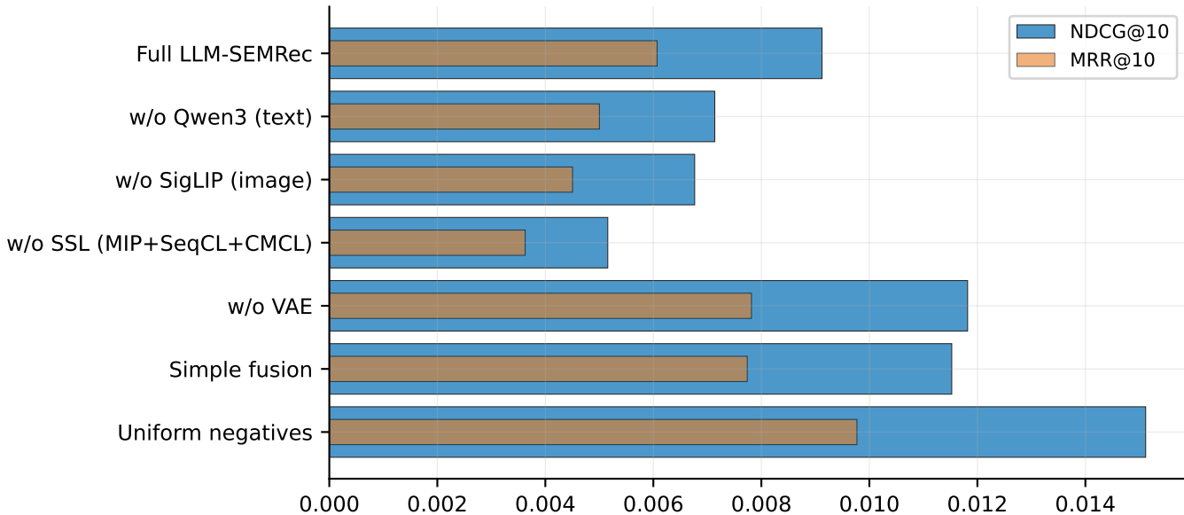
Ablation — NDCG@10 and MRR@10
