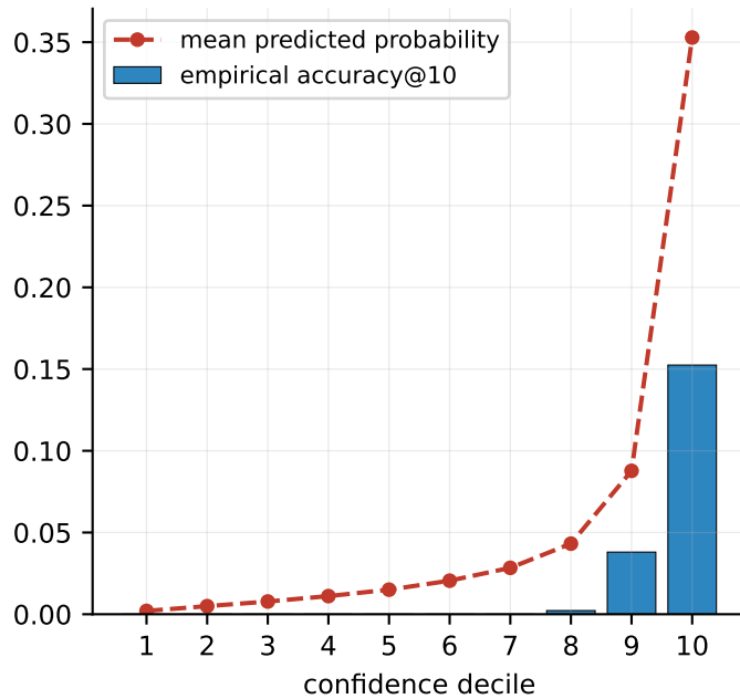
(b) Accuracy vs. predicted confidence
