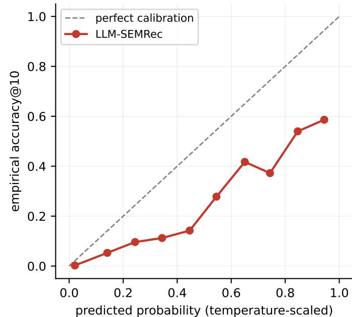
(a) Reliability diagram
