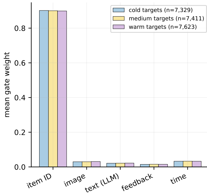
(b) The gate adapts to item popularity
