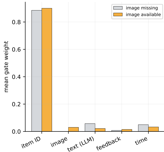
(c) Availability drives the weights (not a zero-valued feature)
