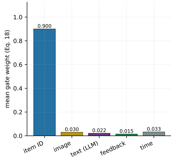
(a) Learned modality importance at the decision position
