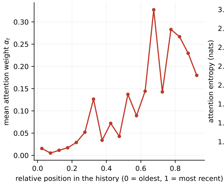
(a) Recency-aware attention profile (Eq. 33-35)
