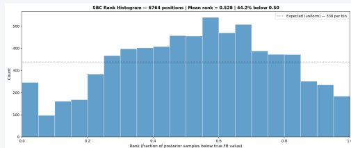
Rank histogram (left)
