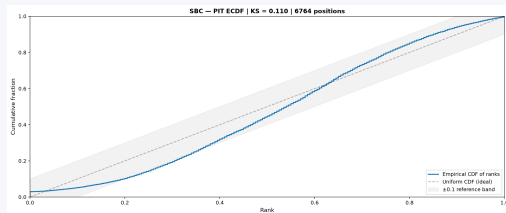
PIT ECDF with KS statistic (right)
