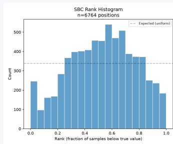
Rank histogram (left)
