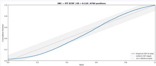
PIT ECDF with KS statistic (right)
