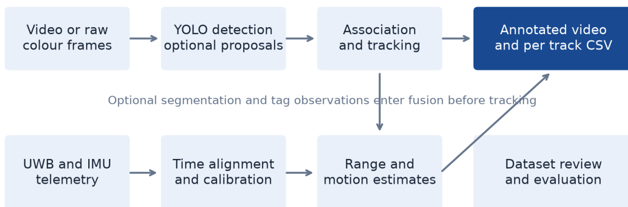
Figure 2. Main data paths reconstructed from run.py , boatdet/pipeline.py , the telemetry scripts and the dataset tools. Optional inputs require their own calibration and validation.
