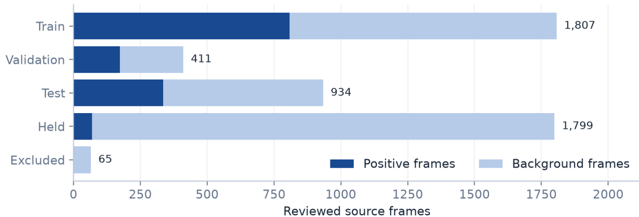
Figure 3. Allocation of the 5,016 reviewed source frames. Held and excluded frames are outside the active train, validation and test datasets. Counts come directly from the frozen manifest.
