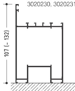
Festfeld Fixed field
