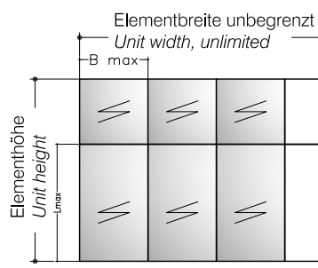
EW30 - Verglasung EW30 - Glazing
