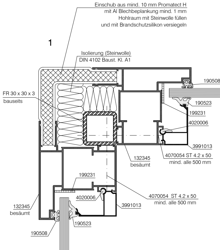
90° Knick horizontal
