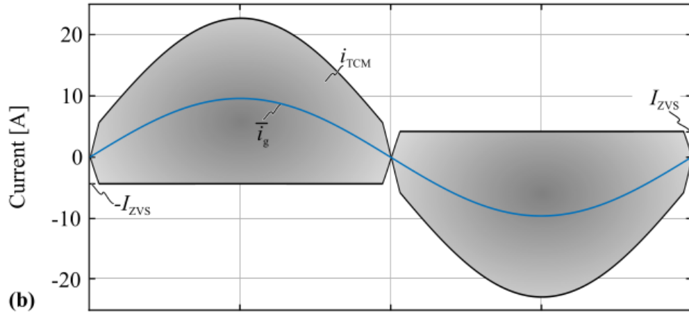
Figure 1.12: iTCM current through L_b
