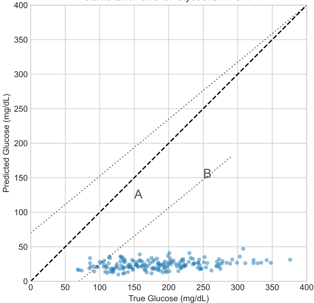
Clarke Error Grid for GlycoSIGHT-CFP
