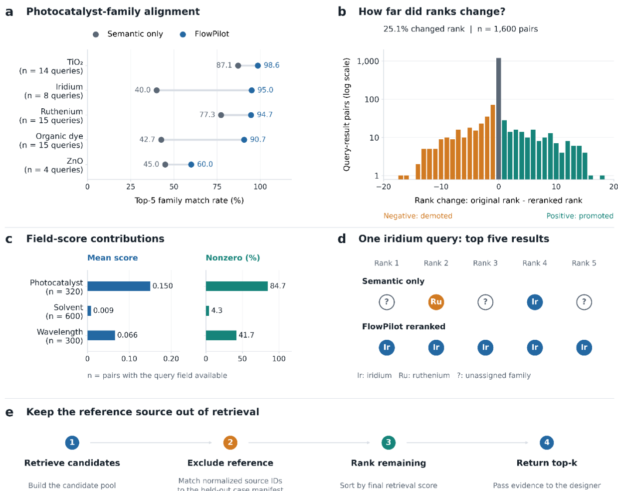
Figure S6. Retrieval alignment and source-exclusion controls. (a) Top-five family match rates, with query counts. (b) Rank change across 1,600 query-result pairs; 401 (25.1%) change rank. The count axis is logarithmic; positive changes indicate promotion. (c) Mean component scores and nonzero percentages among pairs with the query field available. (d) Recorded families for an iridium query: Ir, iridium; Ru, ruthenium; ?, unassigned family, not an established mismatch. (e) Exclusion of normalized held-out source identifiers before final ranking. These metrics assess metadata alignment, not reaction success or absence from model pretraining.
