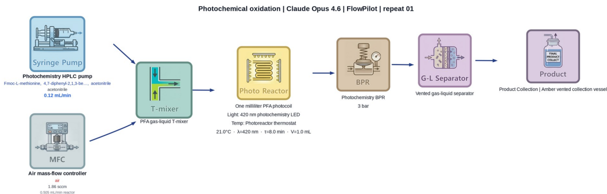
Figure S13. Archived inventory-assigned topology for the Claude Opus 4.6 FlowPilot photochemical-oxidation run, repeat 01. The diagram represents the final structured design, not the unreconciled LLM narrative reproduced below. Its 1.0 mL reactor, 0.12427 mL/min liquid flow and 1.856819 mL/min air feed at inlet/STP correspond to a nominal V_R/Q_L time of 8.046994 min and 1.4 oxygen equivalents. This nominal time is not a measured liquid contact time. The recorded disposition is SCREEN, not experimentally validated execution. The exact one-shot response is preserved in the following subsection and the companion files.
