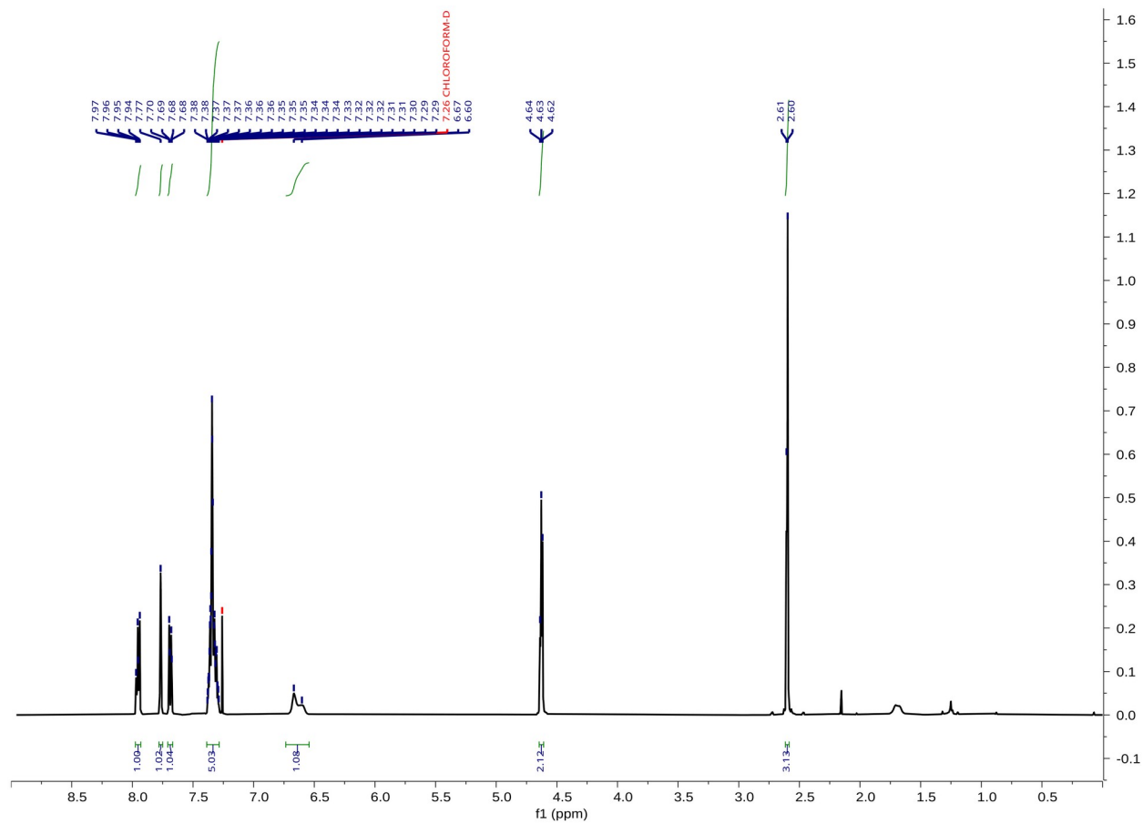
Figure S20. 3b: ^1\text{H} NMR (500 MHz, \text{CDCl}_3 ). Supplied KHU product-characterization spectrum, reproduced without peak reassignment, baseline correction, or deletion of signals.
