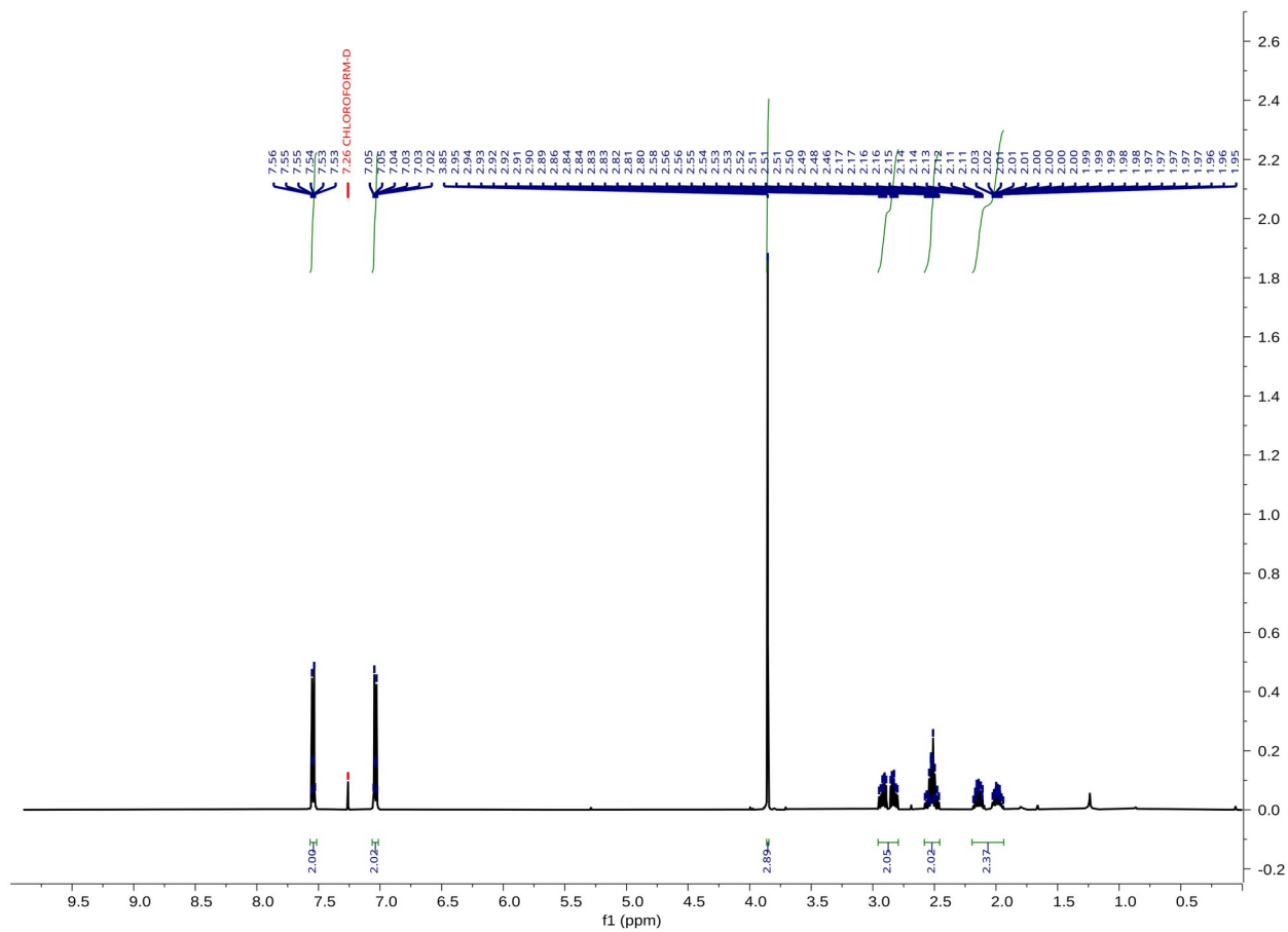
Figure S18. 4a: 1 H NMR (500 MHz, CDCl 3 ). Supplied KHU product-characterization spectrum, reproduced without peak reassignment, baseline correction, or deletion of signals.
