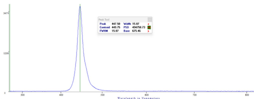
Figure S17. Irradiation sources supplied by KHU: (a) two MR16 5 W batch lamps; (b) Vapourtec 450 nm LED for R1; (c) blue strip LED for R2. The original photographs and emission traces are retained. Reported peak wavelengths are 452.4, 450.32 and 447.50 nm, respectively. Electrical inputs are 5 W per MR16 lamp, 60 W for the Vapourtec source, and 10 W for the strip. The Vapourtec radiant-power specification is 24 W; none of these values establishes irradiance at the reacting fluid.
