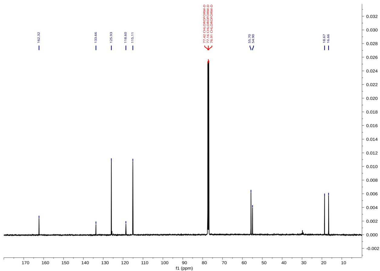
Figure S21. 4a: ^{13}\text{C}\{^1\text{H}\} NMR (126 MHz, \text{CDCl}_3 ). Supplied KHU product-characterization spectrum, reproduced without peak reassignment, baseline correction, or deletion of signals.
