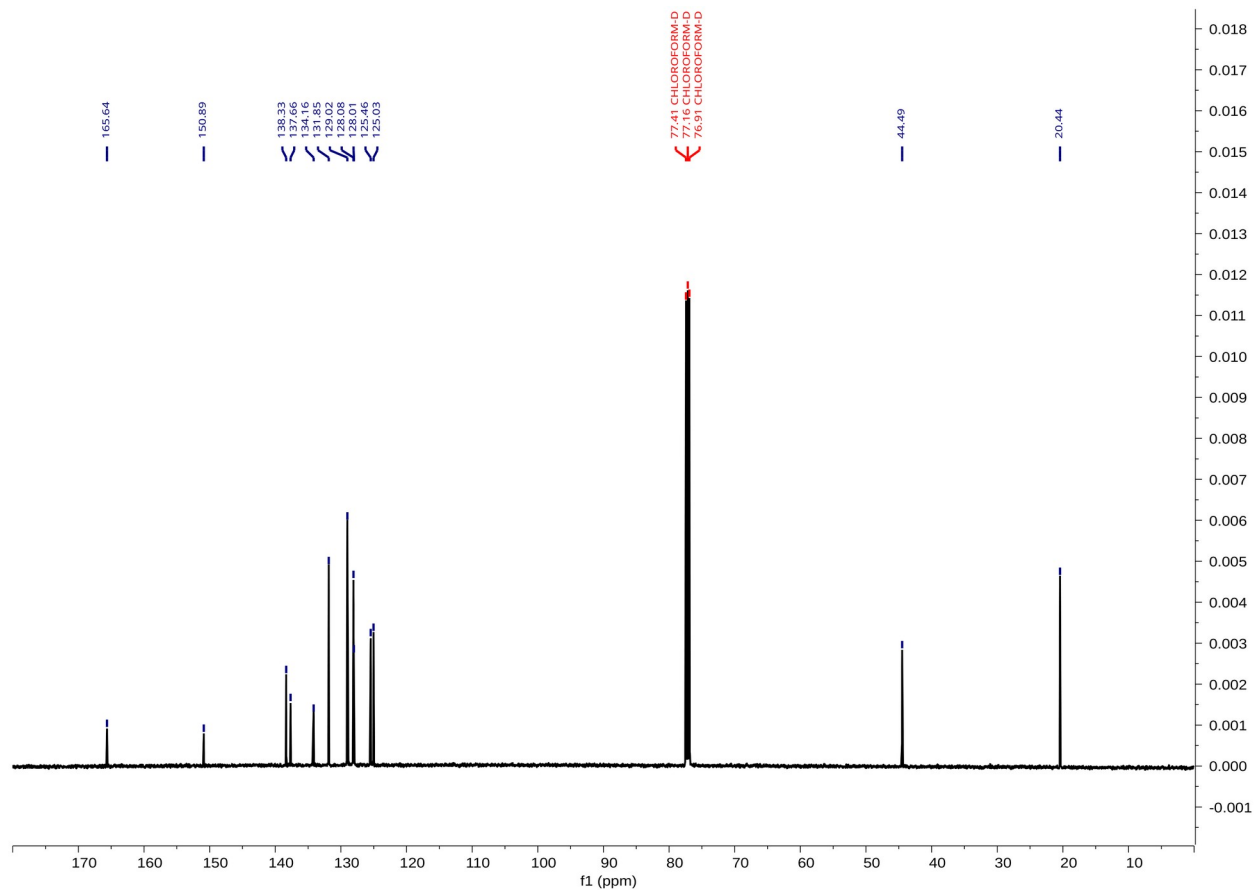
Figure S23. 3b: ^{13}\text{C}\{^1\text{H}\} NMR (126 MHz, \text{CDCl}_3 ). Supplied KHU product-characterization spectrum, reproduced without peak reassignment, baseline correction, or deletion of signals.
