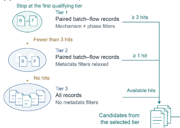
Figure S5. Plan-aware retrieval workflow. (a) ChemistryPlan fields enrich the query before semantic retrieval; an embedding-provider failure invokes the deterministic lexical fallback without changing the query or metadata filters. (b) Tiered retrieval starts with paired records and strict mechanism/phase filters, relaxes filters when fewer than three results remain, and expands to all records only when no paired result remains; hidden source identifiers are excluded. (c) Reranking combines 0.60 semantic similarity with 0.40 field similarity before descending top-k selection.
