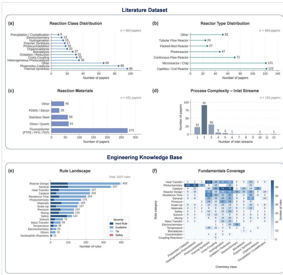
Figure 2. Literature corpus and engineering rule-based coverage. (a-d) Reaction classes, reactor types, reported materials, and inlet-stream configurations in the curated flow-chemistry corpus; explicit inlet-stream counts are available for 154 records. (e) Category and severity distribution within the 2,537-rule engineering knowledge base. (f) Recorded associations between rule categories and chemistry classes. Full categorical exports and field-specific availability are reported in Figures S3–S4 and Tables S4–S5 ; associations indicate knowledge coverage rather than independent validation of every rule.
