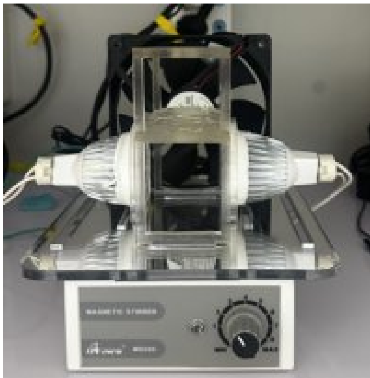
Photo reactor (Batch)
