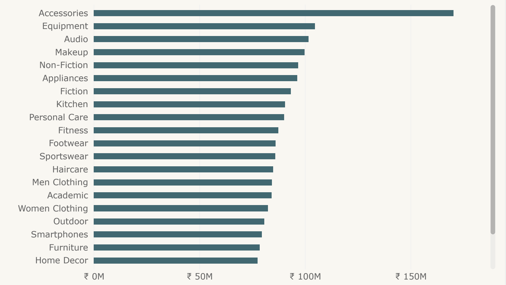
Subcategory Revenue & Profit Margin Health
