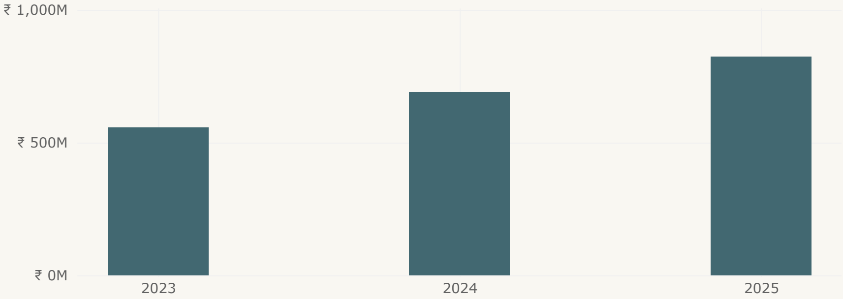
Annual Sales Growth
