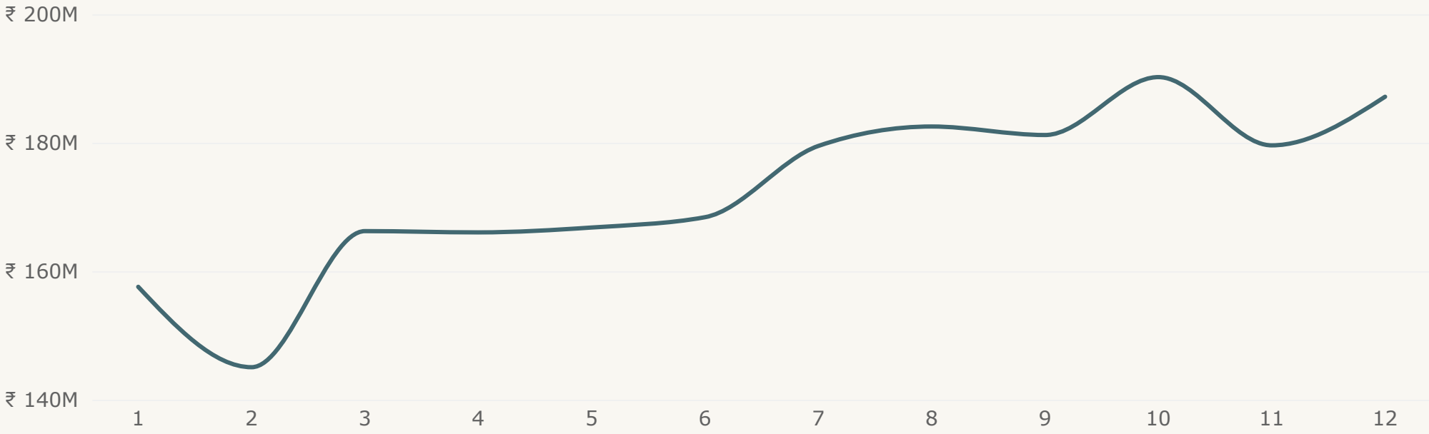
Monthly Seasonality Pattern (Jan-Dec)
