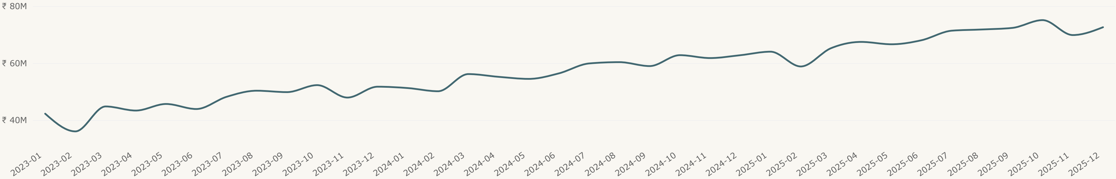
Monthly Sales Trend (2023–2025)
