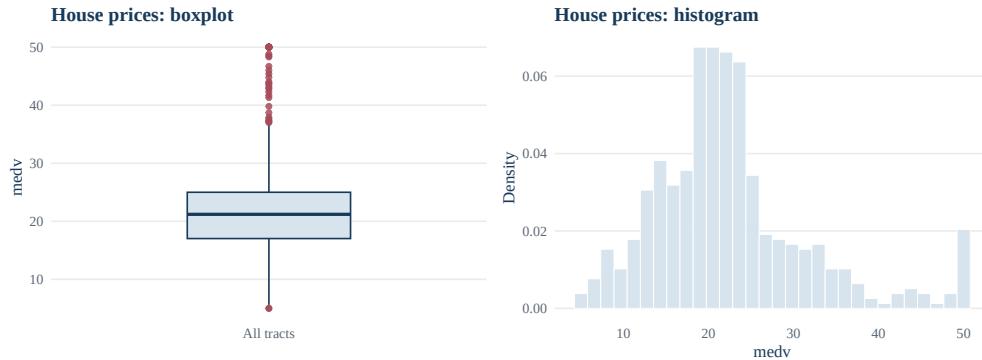
Figure 4: Full-sample distribution of median house values ( medv , in thousands of US dollars) for the 506 census tracts in the MASS::Boston data set. Left panel: boxplot with upper outliers highlighted. Right panel: density-scaled histogram on the same variable.
