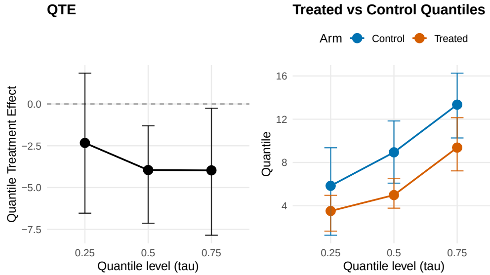
Figure 9: Standardized quantile treatment effect (QTE) summaries for Lalonde 1978 earnings, returned by qte(fit, probs = c(0.25, 0.50, 0.75), interval = "credible") . Left panel: effect curve Q_1^m(\tau) - Q_0^m(\tau) versus \tau with pointwise 95% credible band. Right panel: standardized treated and control quantile curves Q_1^m(\tau) and Q_0^m(\tau) on the original earnings scale, with pointwise credible bands.
