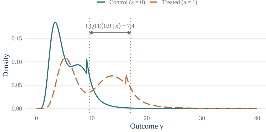
Figure 3: Two arm-specific conditional outcome densities f_a(y | x) , a \in \{0, 1\} , at a representative covariate profile x under a spliced gamma-mixture-plus-GPD model: control arm ( a = 0 , solid) and treated arm ( a = 1 , long-dash). Dotted vertical lines mark the 90th conditional quantiles Q_0(0.9 | x) and Q_1(0.9 | x) , and the double-headed arrow connects them, labelled with the conditional quantile treatment effect CQTE(0.9 | x) = Q_1(0.9 | x) - Q_0(0.9 | x) .
