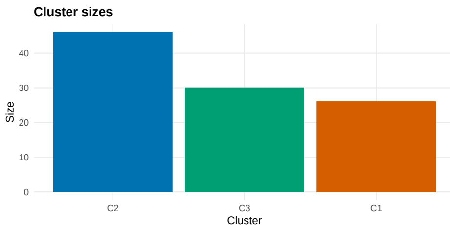
Figure 7: Bar plot of predicted cluster assignments for the held-out Boston test sample (the 20% of medv observations excluded from training), returned by plot(predict(fit_clust, newdata = test_dat, type = "label"), type = "sizes") . Each bar corresponds to one representative training cluster from Figure 6; bar heights give the number of test tracts assigned to that cluster.
