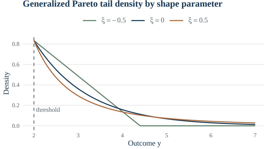
Figure 1: Generalized Pareto distribution (GPD) density above a fixed threshold u = 2 with scale \sigma = 1.2 and three values of the shape parameter, \xi \in \{-0.5, 0, 0.5\} . The dashed vertical line marks the threshold u .
