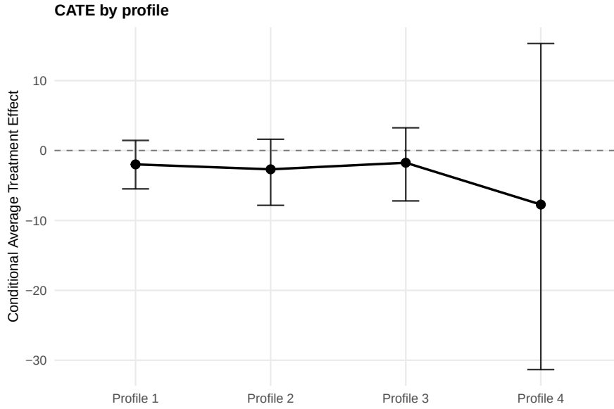
Figure 10: Profile-specific conditional average treatment effects for Lalonde 1978 earnings at the four representative covariate profiles (Profile 1–Profile 4) of Table 4, returned by cate(fit, newdata = xnew, interval = "hpd") . Points denote posterior estimates of \text{CATE}(x) = \mu_1(x) - \mu_0(x) and vertical bars give 95% HPD intervals.
