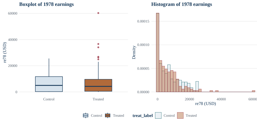
Figure 8: Full-sample distribution of 1978 annual earnings ( re78 , in US dollars) from the MatchIt::lalonde data set, stratified by treatment arm. Left panel: arm-specific boxplots with upper outliers highlighted. Right panel: overlaid density-scaled histograms for the control and treated arms.
