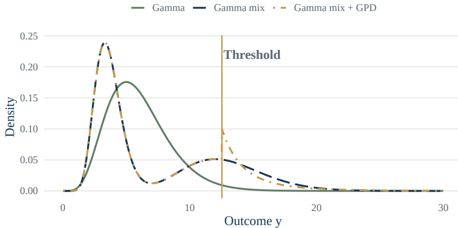
Figure 2: Three density curves on the same axes: a single-component gamma density (solid), a two-component gamma mixture density (long-dash), and a spliced gamma-mixture-plus-GPD density (dot-dash) with GPD tail scale 2.0 and shape 0.25. The vertical line marks the splice threshold, set at the 80th percentile of the two-component gamma bulk mixture.
