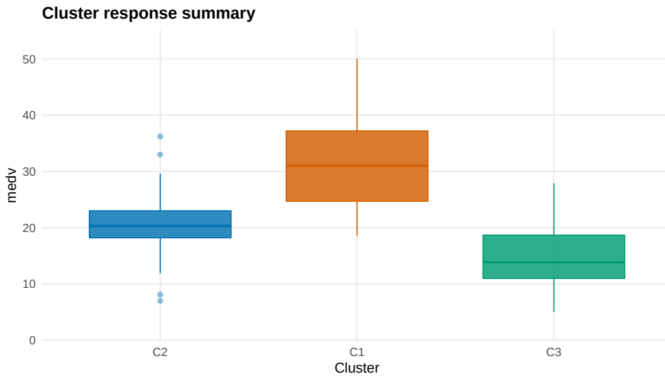
Figure 6: Representative training-cluster summary for the Boston medv analysis, returned by the plot() method applied to the labels object from predict(fit_clust, type = "label") . Training observations are shown on the response scale and coloured by their assigned cluster in the representative partition.
