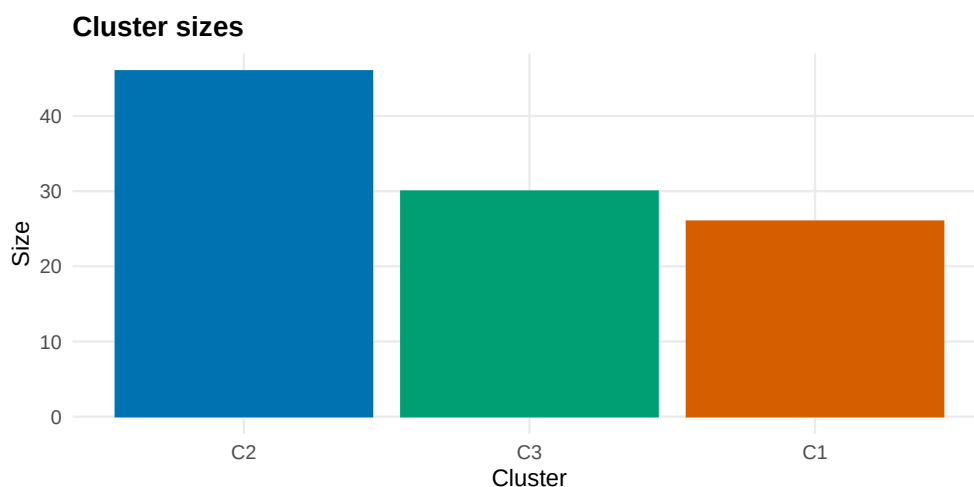
Figure 7: Bar plot of predicted cluster assignments for the held-out Boston test sample (the 20% of medv observations excluded from training), returned by plot(predict(fit\_clust, newdata = test\_dat, type = "label"), type = "sizes") . Each bar corresponds to one representative training cluster from Figure 6; bar heights give the number of test tracts assigned to that cluster.
