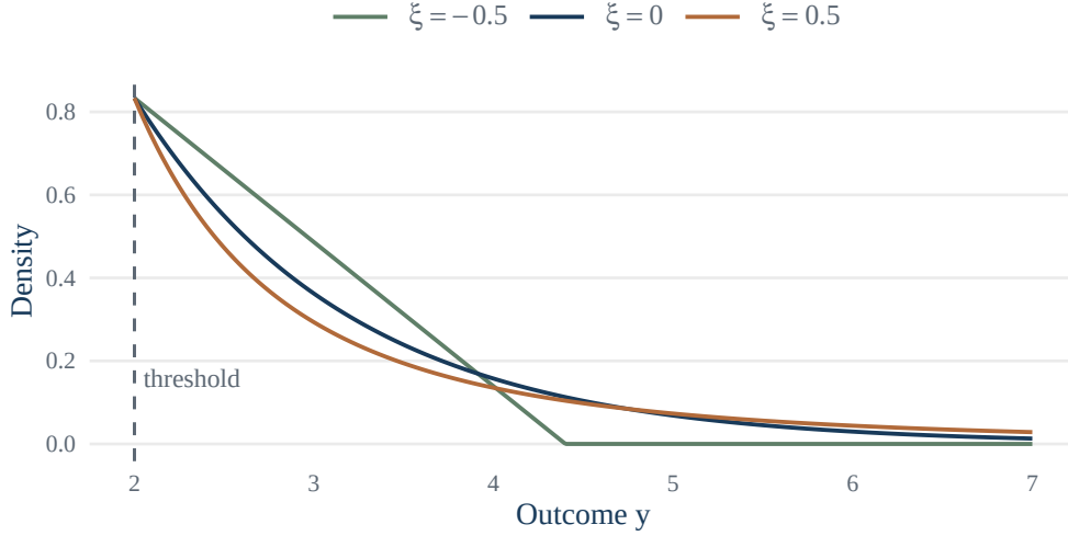
Figure 1: Generalized Pareto distribution (GPD) density above a fixed threshold u = 2 with scale \sigma = 1.2 and three values of the shape parameter, \xi \in \{-0.5, 0, 0.5\} . The dashed vertical line marks the threshold u .
