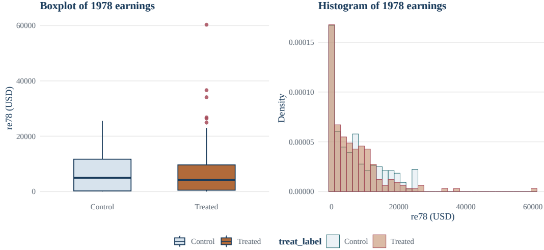
Figure 8: Full-sample distribution of 1978 annual earnings ( re78 , in US dollars) from the MatchIt::lalonge data set, stratified by treatment arm. Left panel: arm-specific boxplots with upper outliers highlighted. Right panel: overlaid density-scaled histograms for the control and treated arms.
