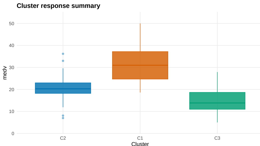
Figure 6: Representative training-cluster summary for the Boston medv analysis, returned by the plot() method applied to the labels object from predict(fit\_clust, type = "label") . Training observations are shown on the response scale and coloured by their assigned cluster in the representative partition.
