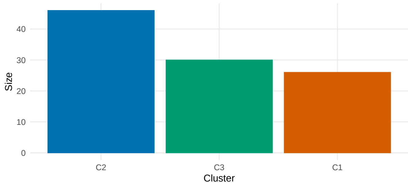
Cluster sizes
