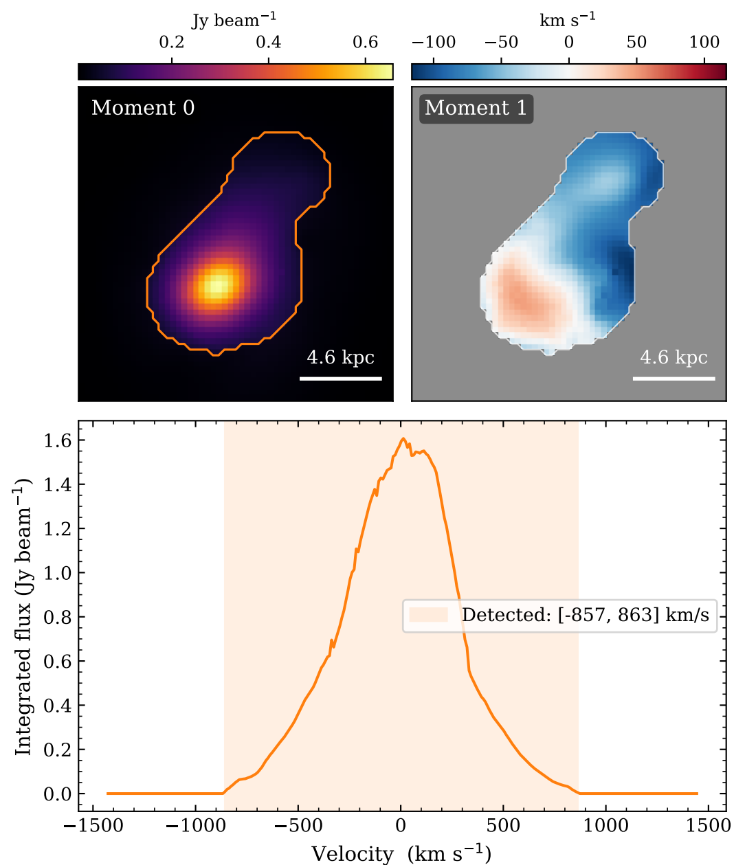
Source 2 | pixel (73, 76) RA 341.53143 Dec -5.44294
