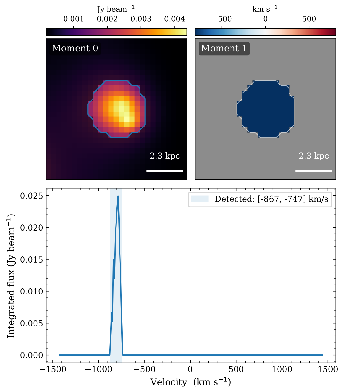
Source 1 | pixel (103, 98) RA 341.53101 Dec -5.44263
