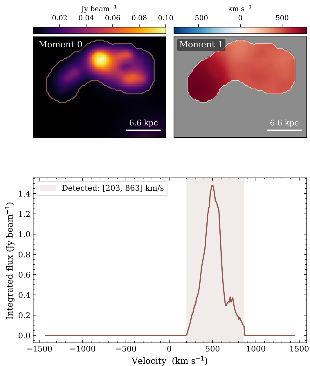
Source 4 | pixel (46, 117) RA 341.53181 Dec -5.44237
