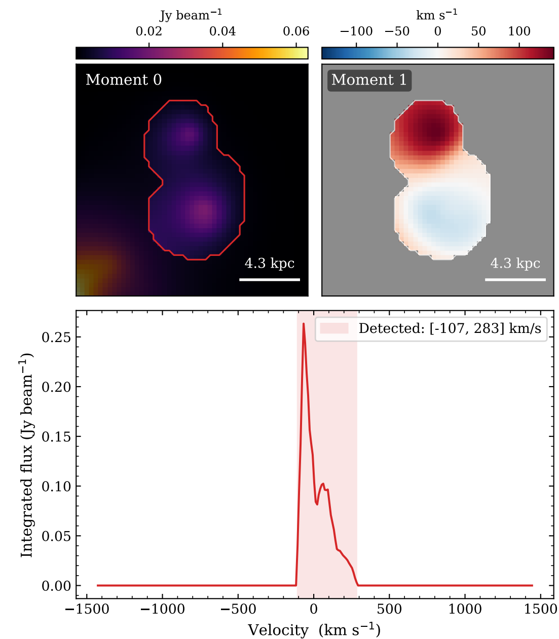
Source 3 | pixel (102, 105) RA 341.53102 Dec -5.44254
