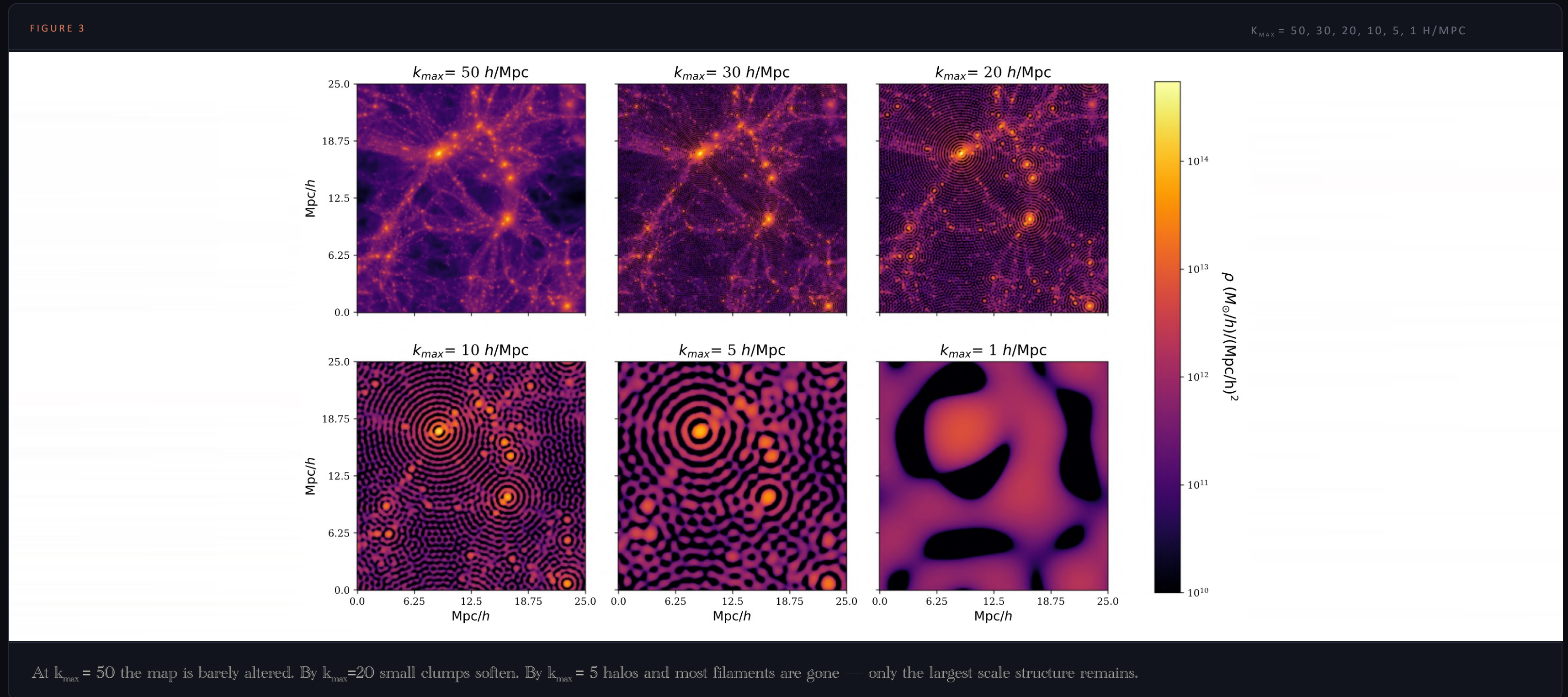
Figure 3 — the maps at decreasing k_{\max} .
