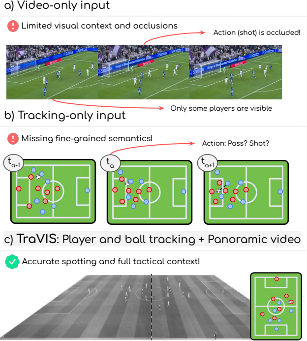
Figure 1: Illustration of standard football action spotting approaches: (a) video-only inputs suffer from limited visual context and severe occlusions, often missing players outside the frame; whereas (b) tracking-only inputs capture the global tactical layout but lack the fine-grained visual semantics crucial for distinguishing specific actions (e.g., a pass versus a shot). In contrast, (c) TRAVIS fuses panoramic video—shown in grayscale for anonymization purposes only—with 2D player and ball tracking, effectively combining precise visual cues with full tactical context for precise action spotting.
