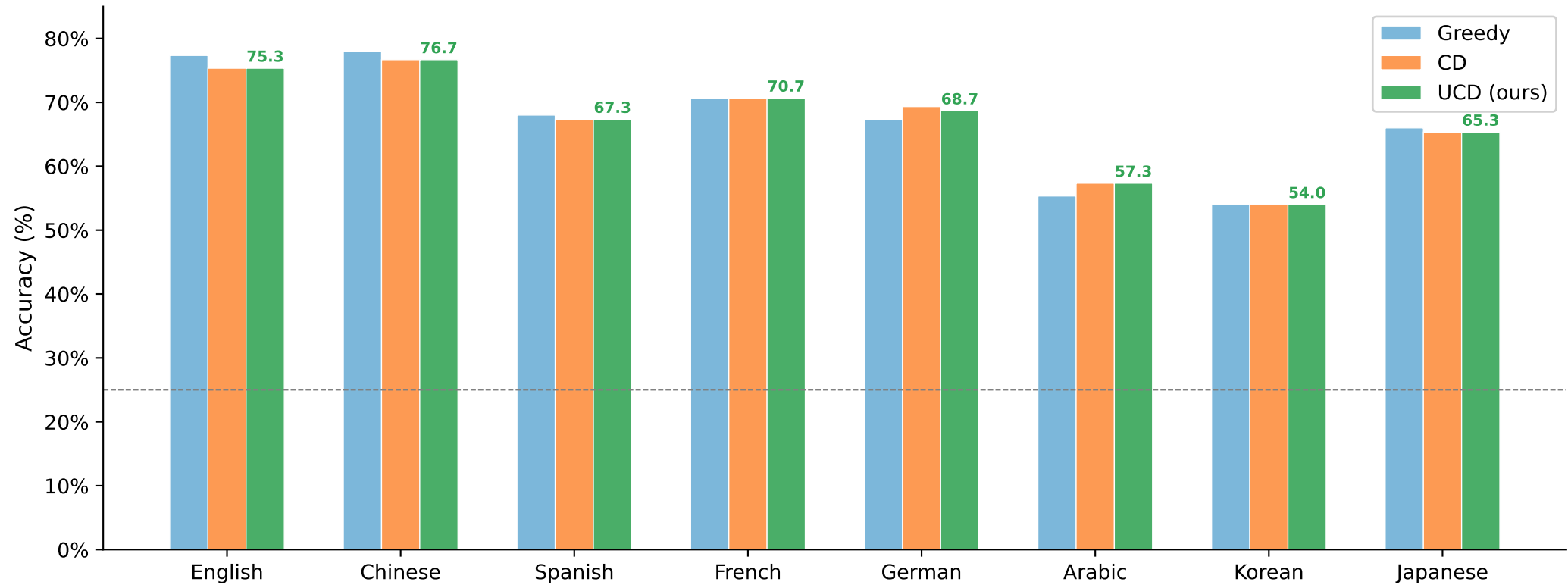
UCD vs. Baselines on Multilingual Medical QA (MMMLU-Medical)
