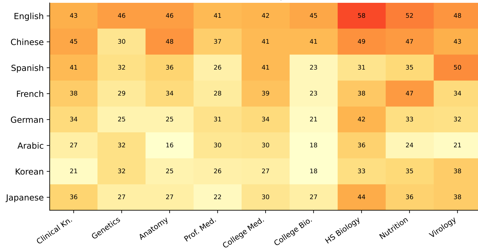
Greedy
