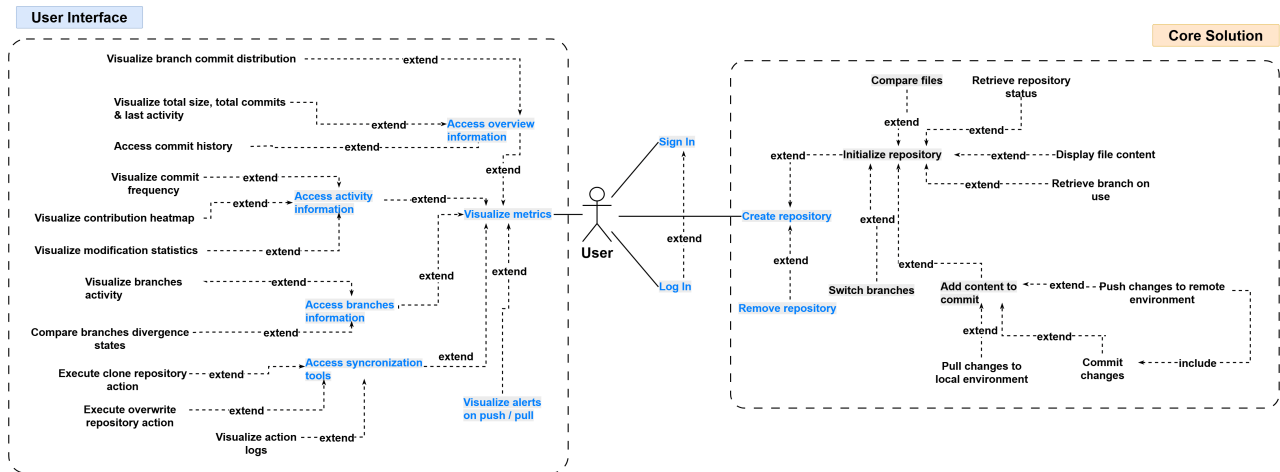
Fig. 4: User use case actions overview.
