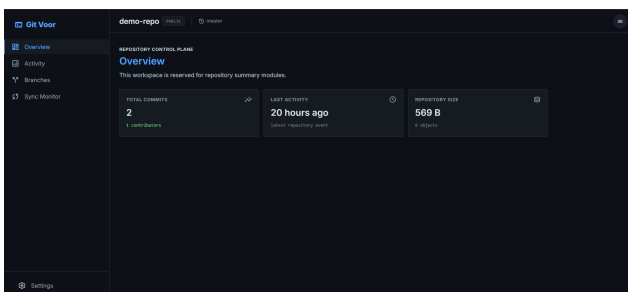
Fig. 10: Overview screen.
