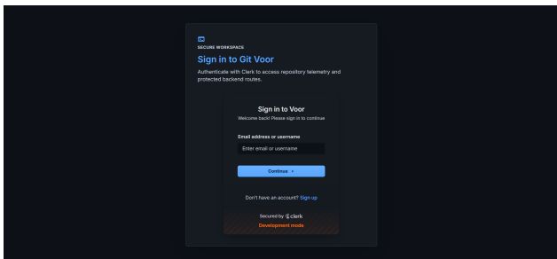
Fig. 8: Login screen.
