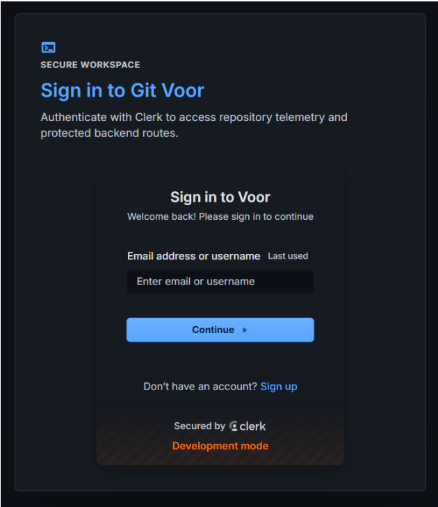
Fig. 8: Login screen.
