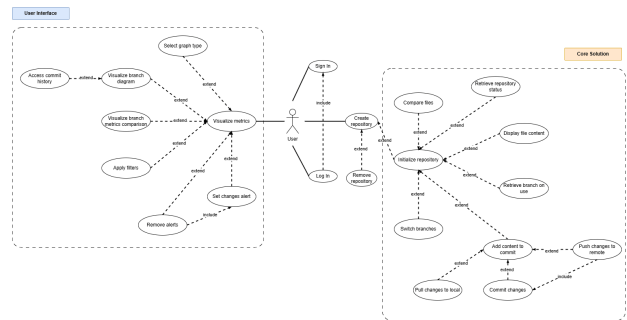
Fig. 5: User use case actions overview.
