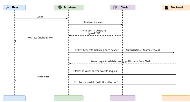
Fig. 7: Sequence diagram auth in Clerk.
