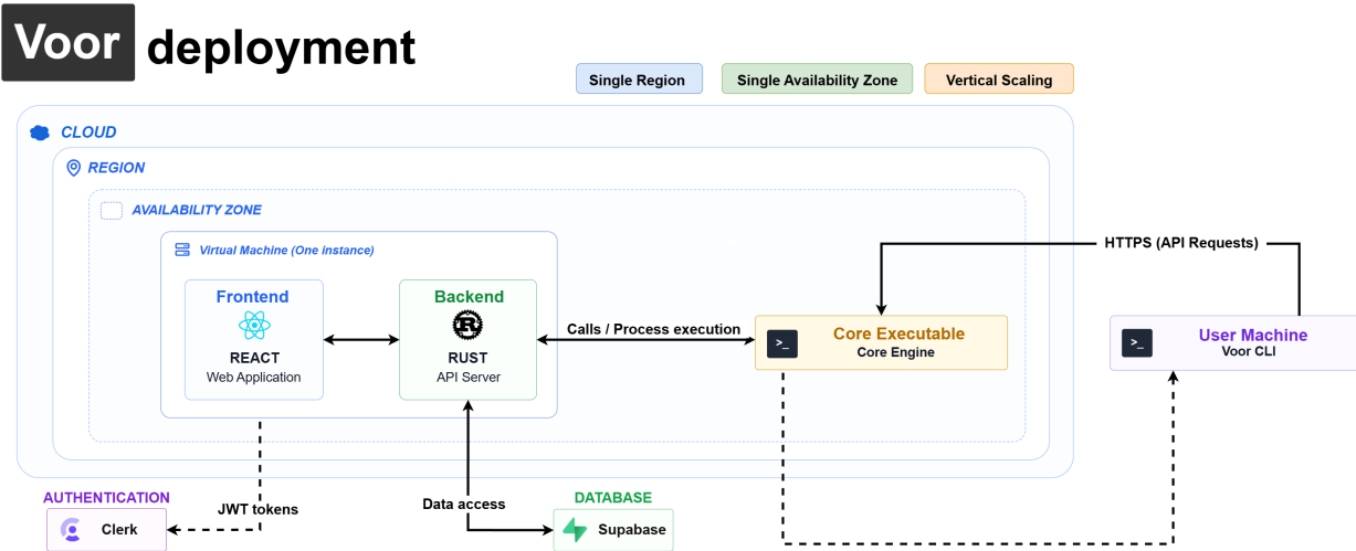
Fig. 2: High-level deployment architecture describing the main components and services that would form the Voor system environment.
