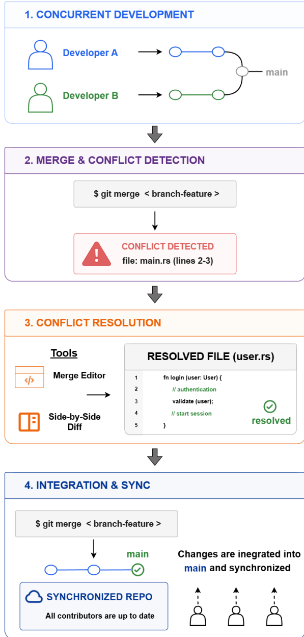
Fig. 2: Collaborative environments workflow.
