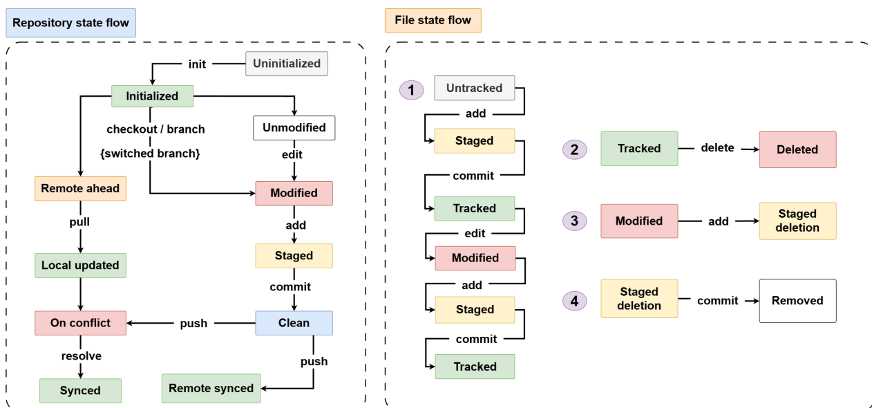
Fig. 5: Repository and file state flow illustrating internal data transitions.
