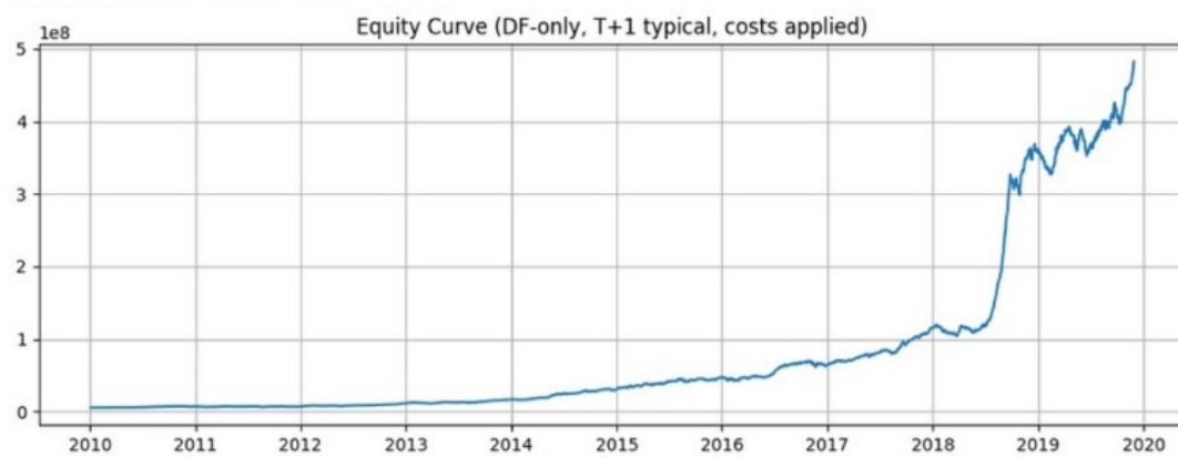
Figure 1: Equity curve from 2010 to 2020.
