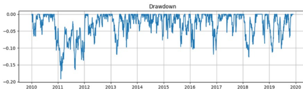
Figure 2: Portfolio drawdown behavior over the full backtest period.
