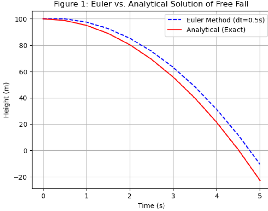
Figure 1: Euler method approximation vs. the analytical solution for free-fall height over time ( \Delta t = 0.5s ).
