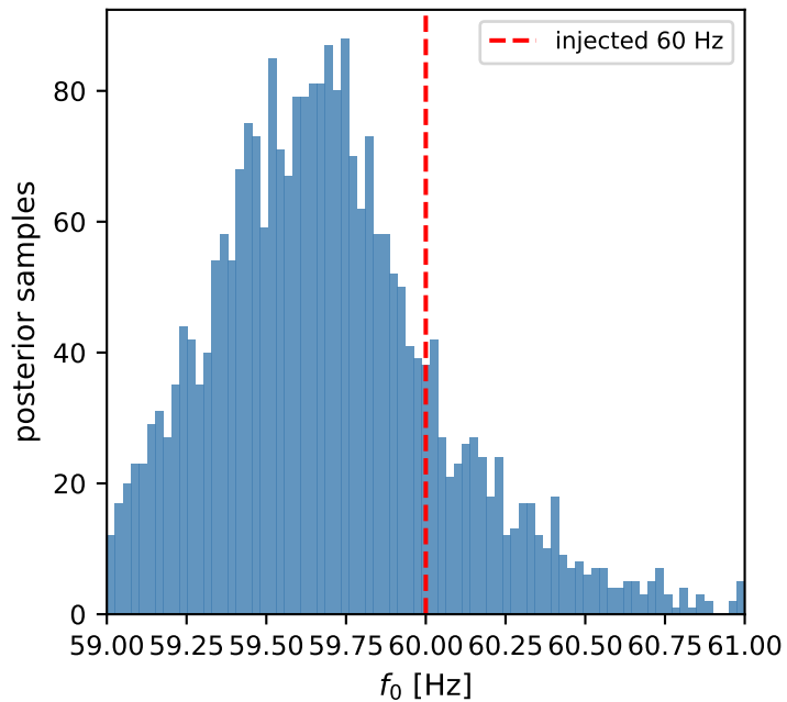
(b) Stage 1b: f_0 recovered < 1 Hz
