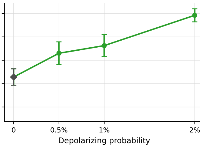
Depolarizing Noise
