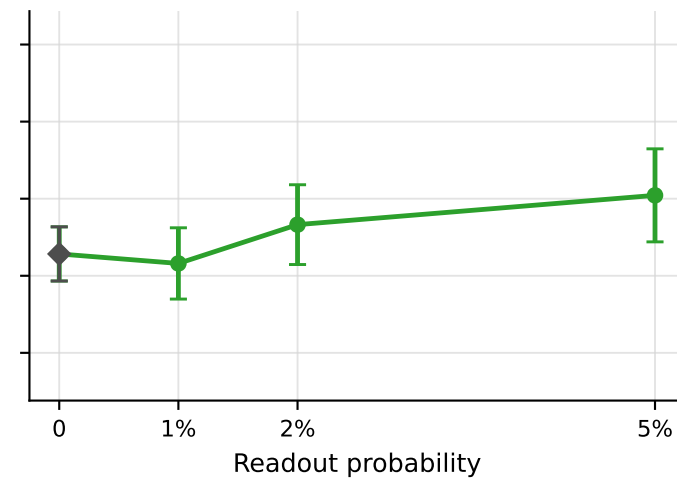
Readout Noise
