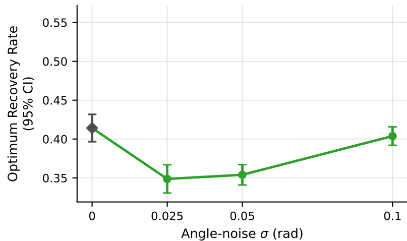
Angle Noise
