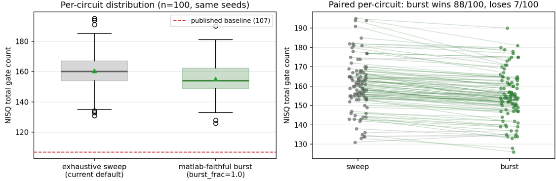
Figure 9: NISQ cost-aware total gate count, exhaustive sweep versus the matlab_demo-faithful burst reducer, n = 100 , identical seeds. Left: per-circuit distribution against the published baseline. Right: paired per-circuit change, colored by direction.
