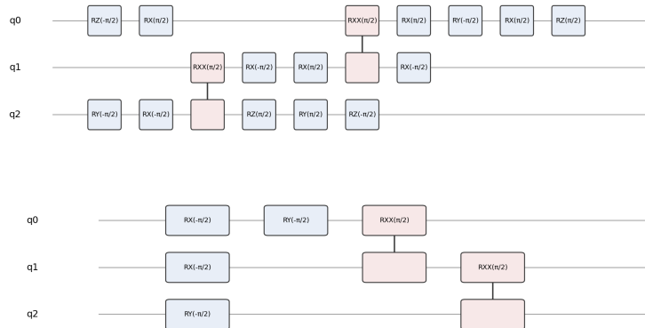
Figure 1: A random 16-gate ion-trap circuit reduced to 6 gates by the exact engine, verified unitary-equivalent to machine precision.
