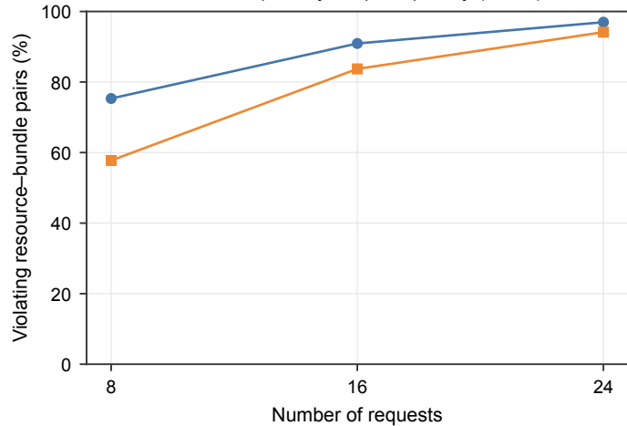
Minimum penalty-drop frequency ( \delta = 1 )
