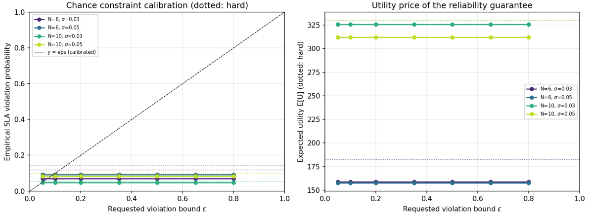
Figure 12: Chance-constrained routing: empirical SLA-violation probability versus requested \epsilon (left; dotted: hard, diagonal: calibrated) and expected utility versus \epsilon (right). The hard rule’s implicit risk is 5–14%.
