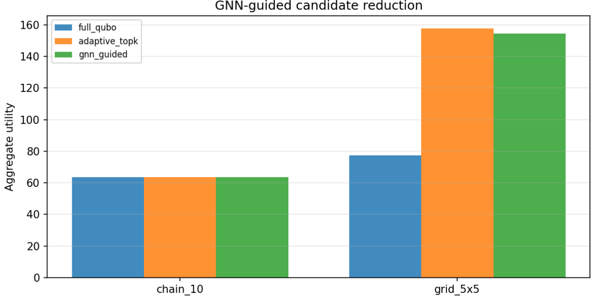
Figure 10: Aggregate utility of full-QUBO, adaptive top- k , and GNN-guided candidate reduction.
