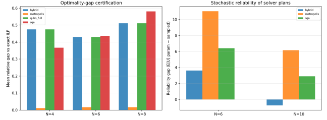
Figure 11: Optimality certification: mean relative gap versus exact ILP (left) and reliability gap of solver plans (right).
