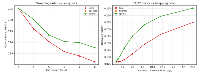
Figure 15: Delivered fidelity of linear, balanced, and optimal swap trees versus path length (left) and memory coherence time (right).
