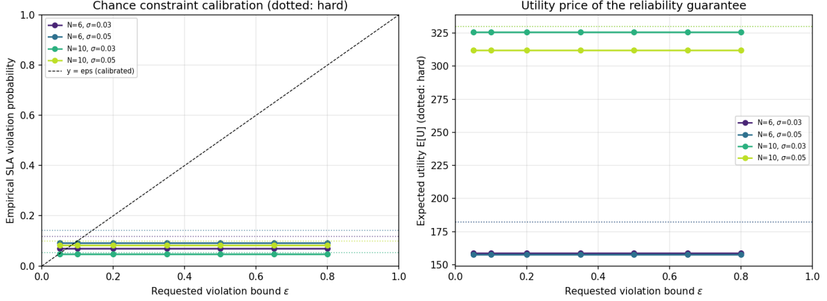
Figure 12: Chance-constrained routing: empirical SLA-violation probability versus requested \varepsilon (left; dotted: hard, diagonal: calibrated) and expected utility versus \varepsilon (right). The hard rule’s implicit risk is 5–14%.
