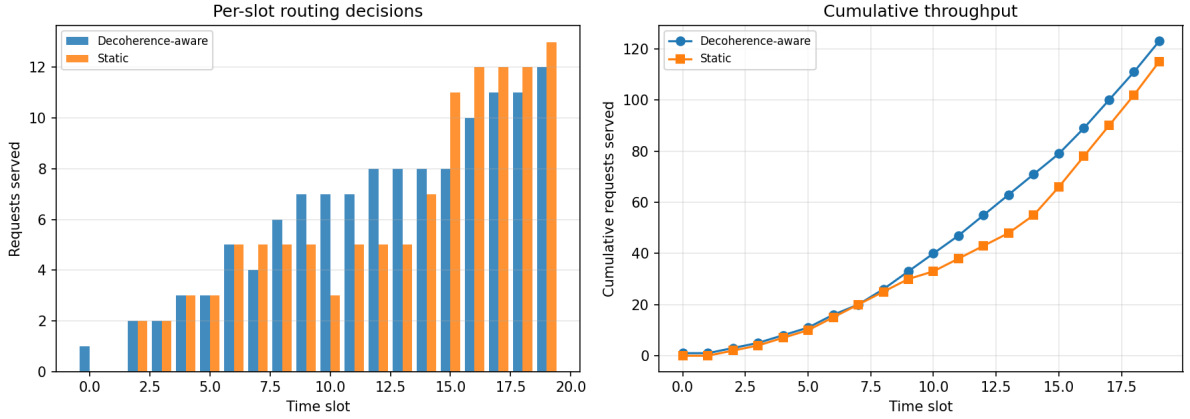
Figure 20: Per-slot (left) and cumulative (right) served requests for the decoherence-aware and static routers on the shared Poisson trace of Table 9.
