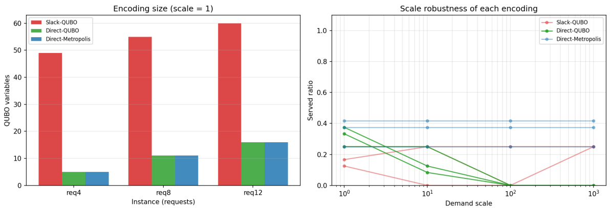
Figure 5: Hamiltonian encoding comparison. Left: QUBO variable count per formulation at scale 1—the direct (slack-free) formulation uses 5–16 binaries vs. 49–60 for the slack-variable encoding. Right: served ratio vs. demand scale; the direct formulation dominates at moderate scales.
