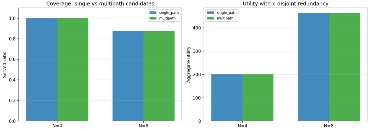
Figure 17: Coverage (left) and utility (right) of single-path versus k -disjoint multipath candidate sets.
