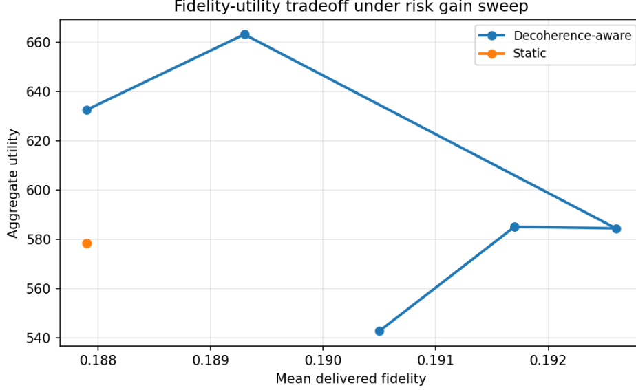
Figure 21: Fidelity-utility tradeoff of the decoherence-aware router as the risk weight \lambda_g is swept ( \lambda_g \in \{0, 0.25, 0.5, 1, 2, 4\} ). The static router is a single point; the risk-aware router traces a Pareto frontier that dominates it.
