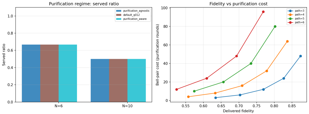
Figure 14: Purification as a first-class variable: regime comparison (left) and fidelity/utility sweep over purification rounds and path length (right).
