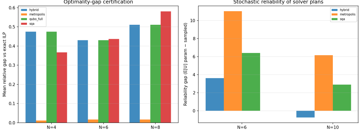
Figure 13: Optimality certification: mean relative gap versus exact ILP (left) and reliability gap of solver plans (right).
