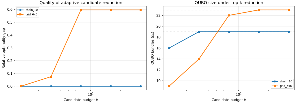
Figure 8: Relative optimality gap (left) and QUBO size (right) versus per-request candidate budget k on chain and grid topologies.
