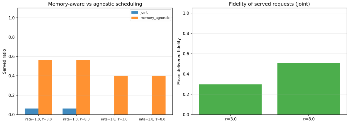
Figure 6: Memory-aware versus memory-agnostic scheduling: served ratio (left) and mean delivered fidelity of the joint router (right) across mean rates and coherence times.
