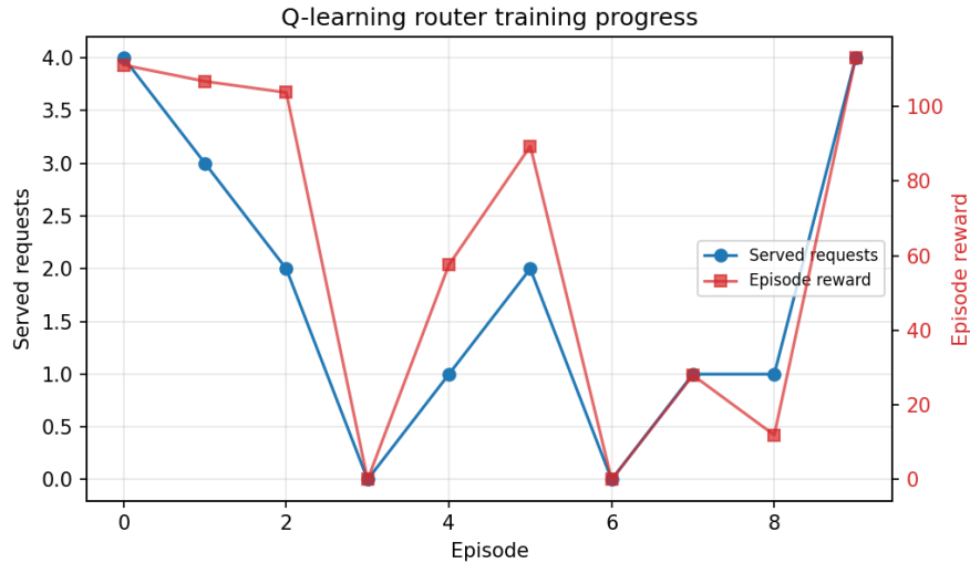
Figure 23: Training progress of the tabular Q-learning router: served requests per episode (left axis) and episode reward (right axis) over 10 training episodes.
