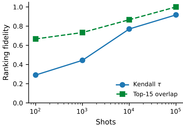
Acquisition-ranking fidelity vs. shots
