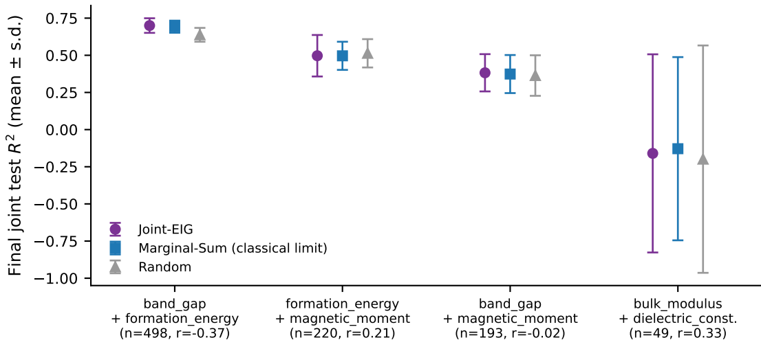
Joint-EIG vs. classical limit vs. random, four real property pairs
